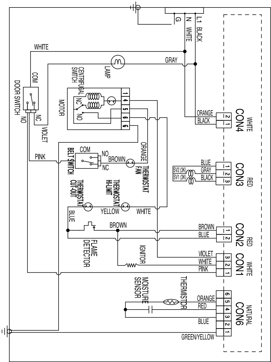
WIRING DIAGRAM : GAS Dryer
